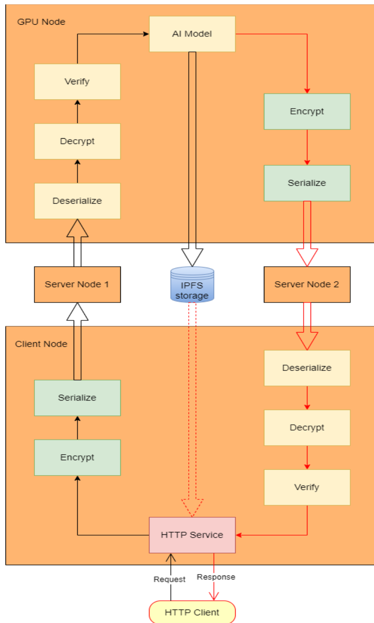
System Technical Architecture Diagram and Code Logic Diagram
